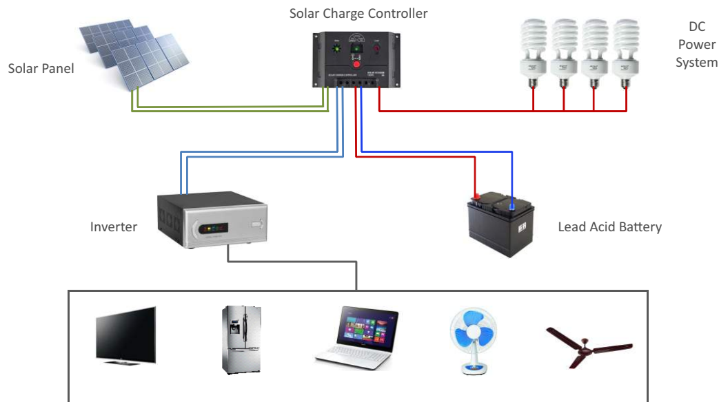
Solar Power Pack with Battery Backup (Off Grid Type) (Range: 240 W to 10 kW)
